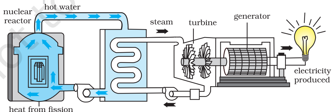
Fig. 3.17 : Nuclear Energy
